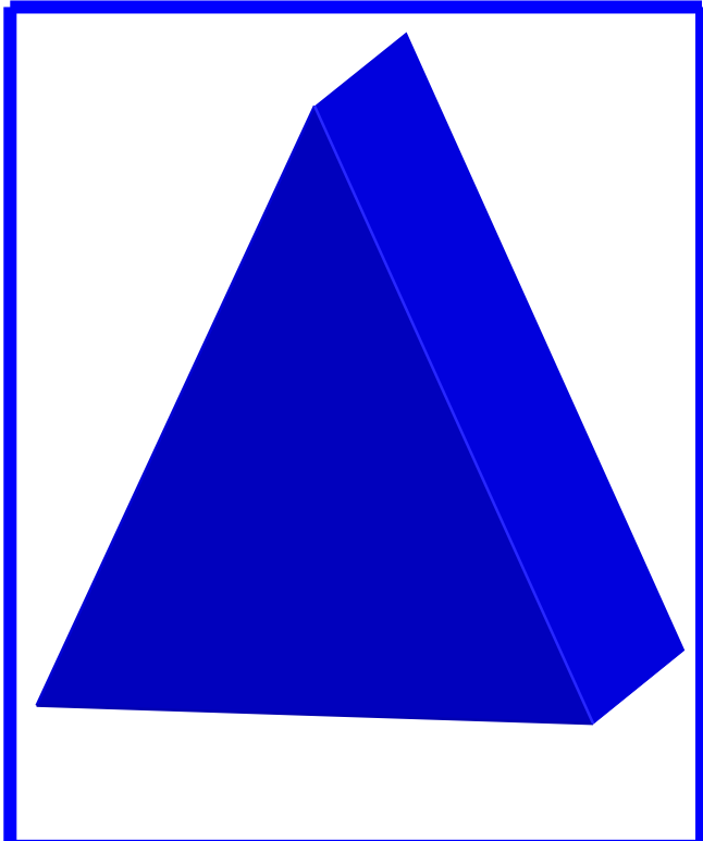
equilateral triangle
