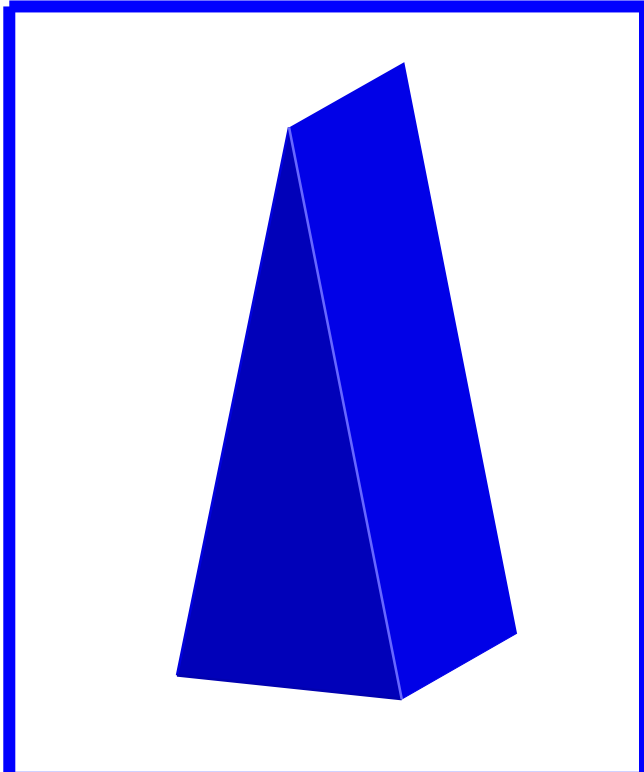
isosceles triangle
